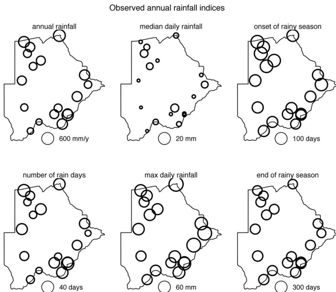
Figure 3.1: Observed distribution of rainfall indices in Botswana.
