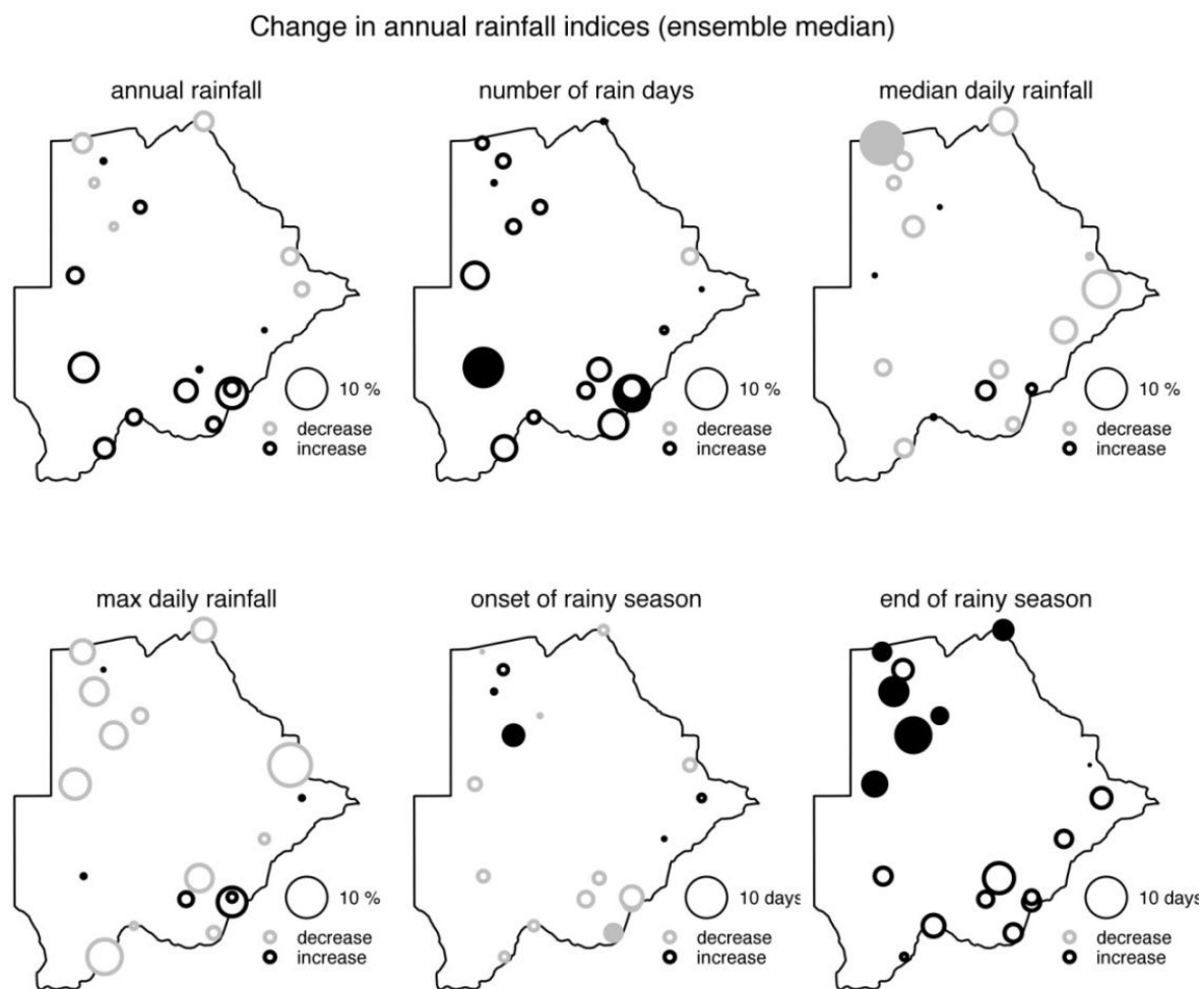
Figure 3.2: Projected distribution of rainfall indices in Botswana, 2046-2065.
