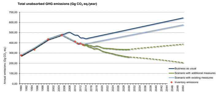
Estimation of unabsorbed GHG emissions for the different mentioned scenarios.
