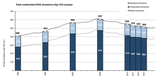
Greenhouses gases emissions in Andorra (1990-2013)
