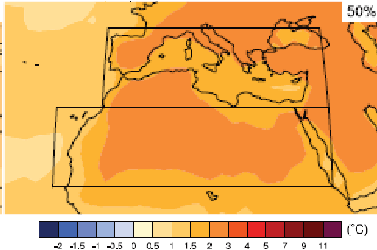
Temperature change RCP4.5 in 2046–2065: June–August
