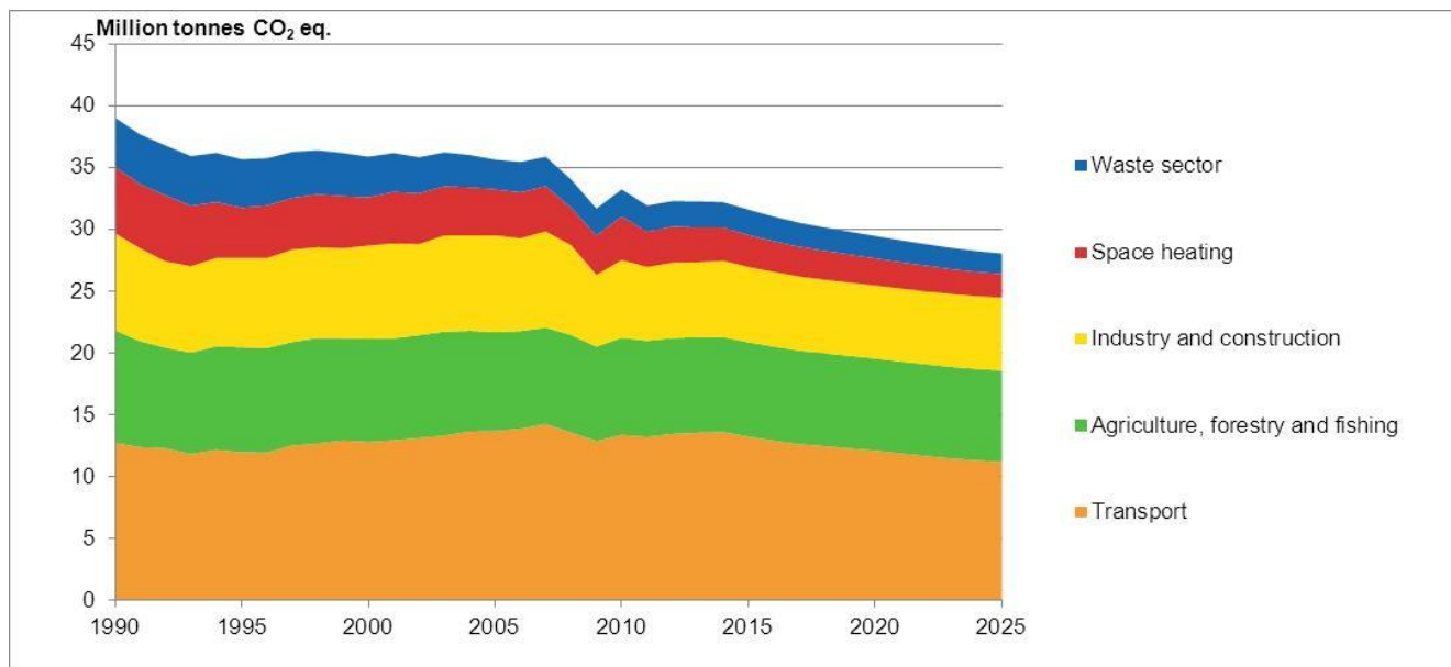
Figure 5.4 Emissions in the non-ETS sector by category (1990–2011) based on the latest greenhouse gas inventory and the WM projection (up to 2025)
