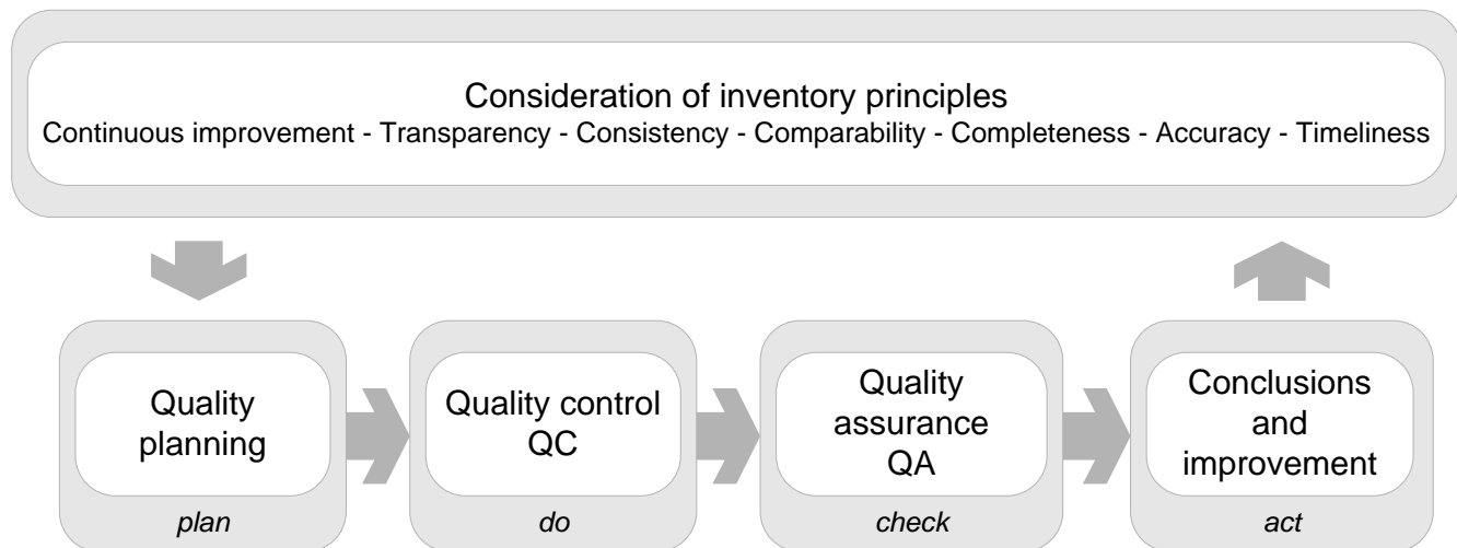
Figure 2.8 QA/QC process concerning preparation of the national greenhouse gas inventory
