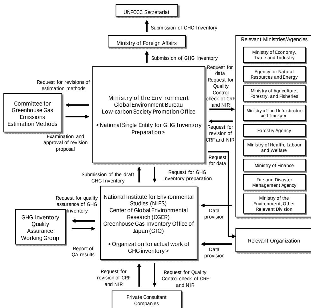
Figure 1-22 Japan's Institutional Arrangements for the National Inventory Preparation
