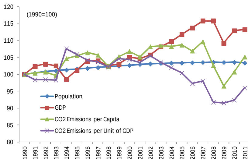
Figure 1-8 Trends in Population, GDP, CO 2 Emissions per Capita, CO 2 Emissions per Unit of GDP (FY1990=100)
