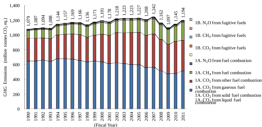
Figure 1-15 Trends in GHG Emissions from the Energy Sector
