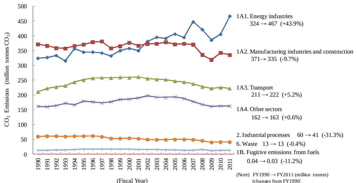
Figure 1-3 Trends in CO 2 Emissions in Each Sector
