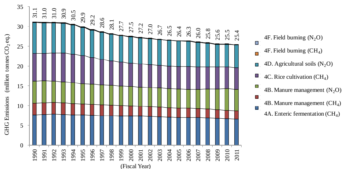
Figure 1-18 Trends in GHG Emissions from the Agriculture Sector
