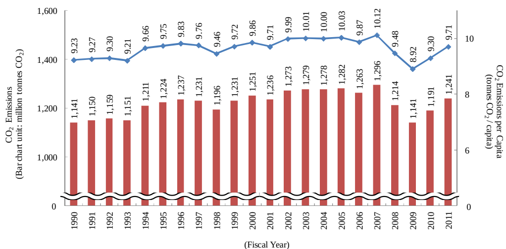
Figure 1-6 Trends in Total CO 2 Emissions and CO 2 Emissions per Capita
