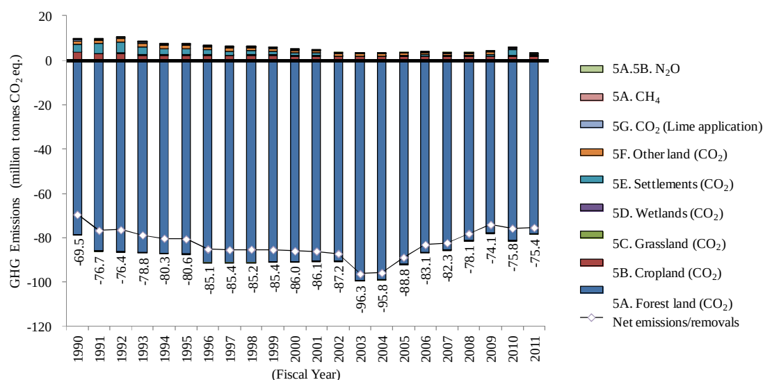
Figure 1-19 Trends in GHG Emissions and Removals from the LULUCF Sector
