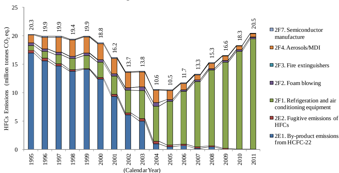
Figure 1-11 Trends in HFCs Emissions
