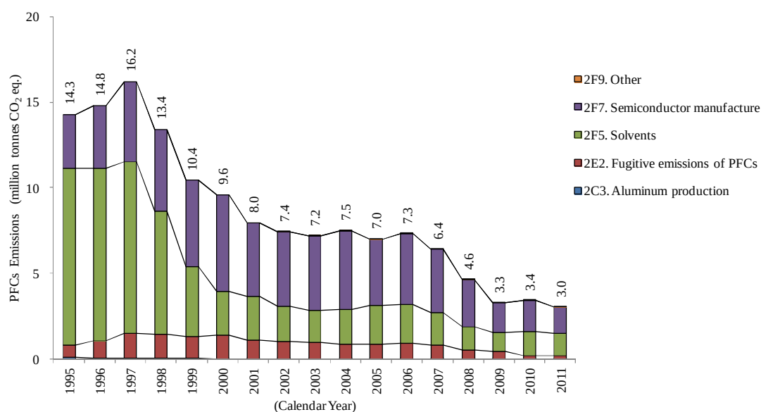
Figure 1-12 Trends in PFCs Emissions
