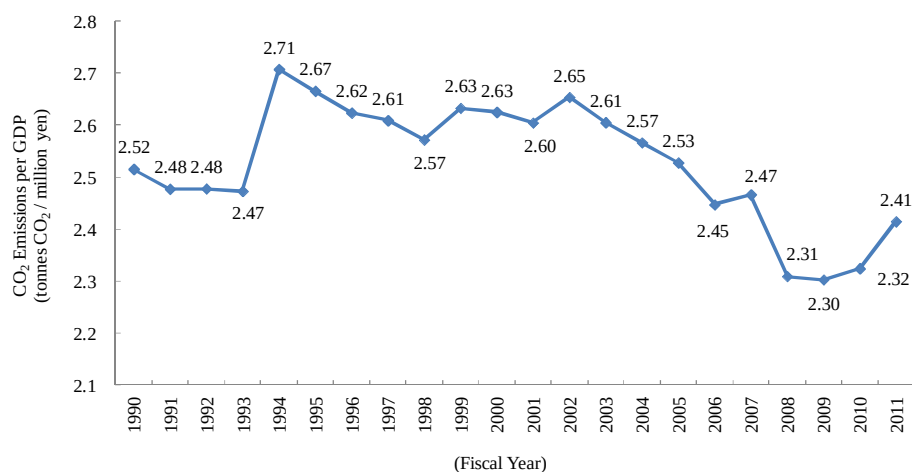
Figure 1-7 Trends in CO 2 Emissions per Unit of GDP
