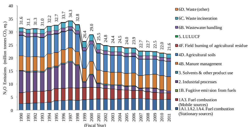
Figure 1-10 Trends in N 2 O Emissions
