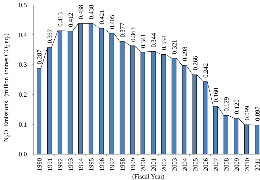
Figure 1-17 Trends in GHG Emissions from the Solvent and Other Product Use Sector
