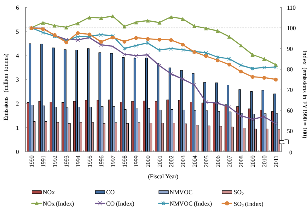
Figure 1-21 Trends in Emissions of Indirect GHGs and SO 2
