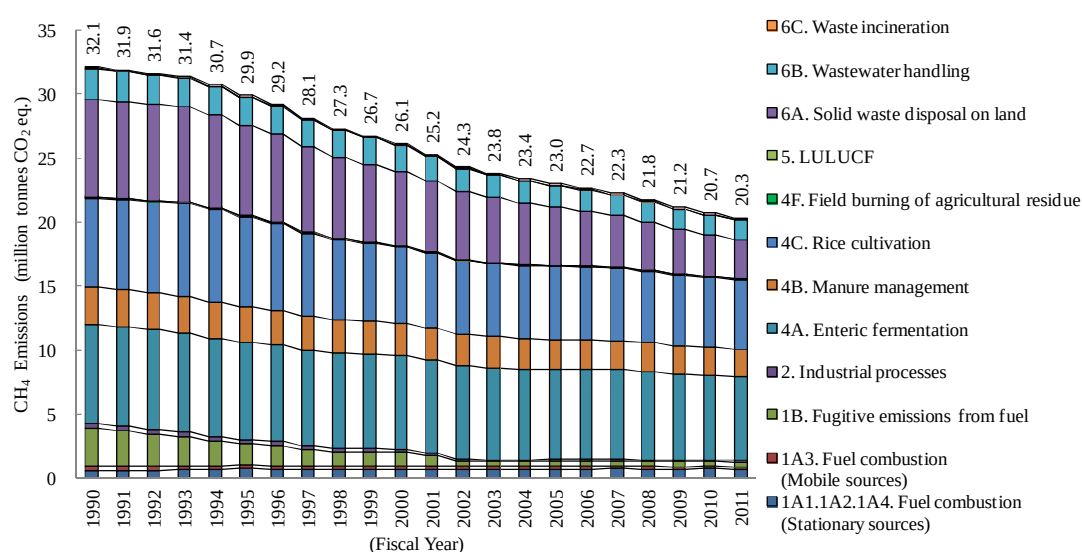
Figure 1-9 Trends in CH 4 Emissions
