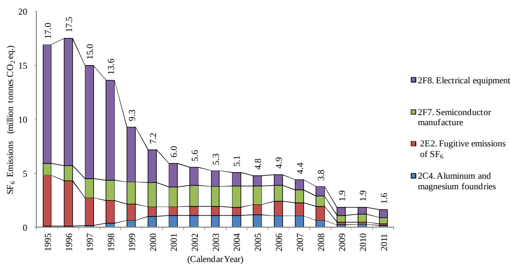
Figure 1-13 Trends in SF 6 Emissions
