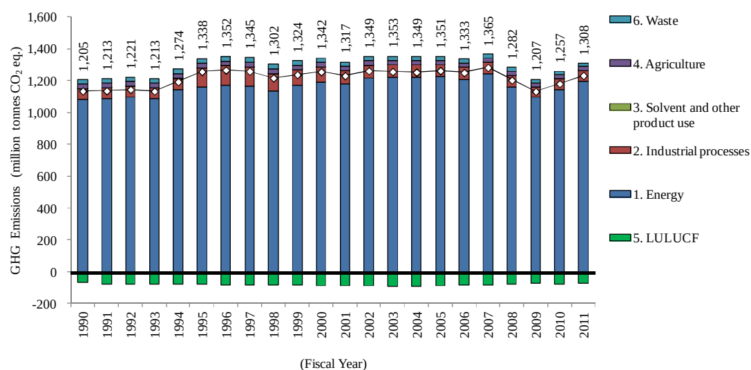
Figure 1-14 Trends in GHG Emissions and Removals in Each Sector
