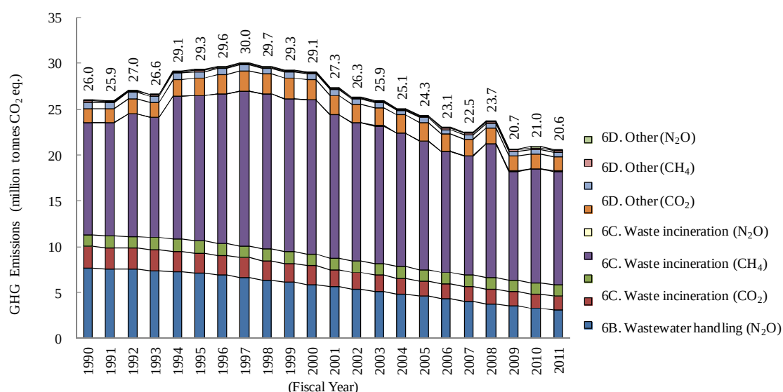
Figure 1-20 Trends in GHG Emissions from the Waste Sector
