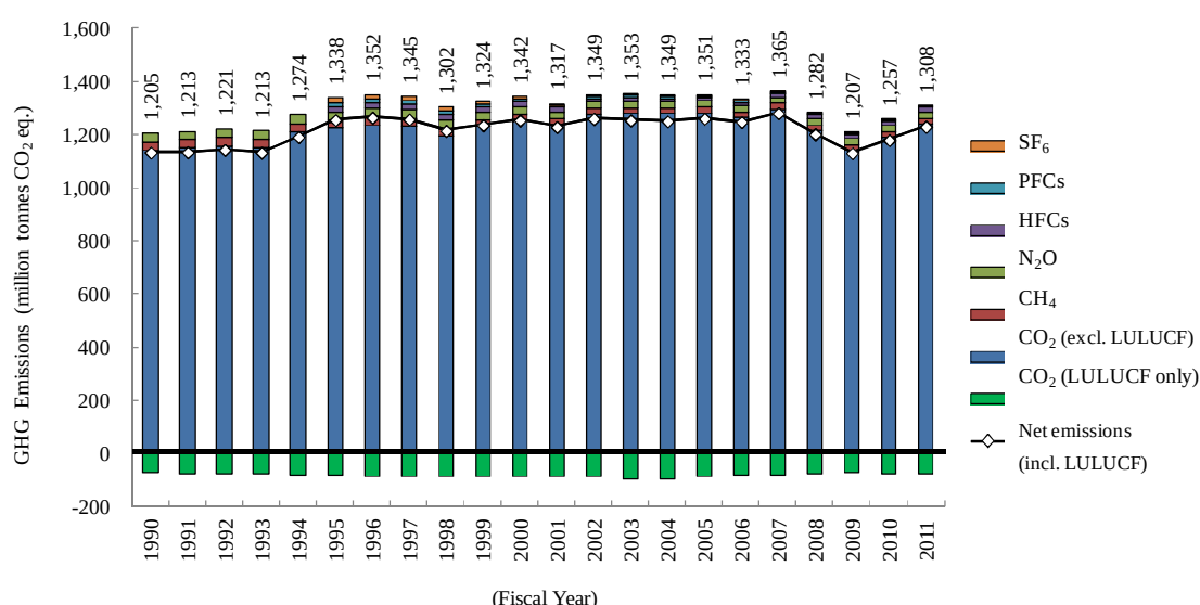
Figure 1-1 Trends in GHG Emissions and Removals in Japan 6
