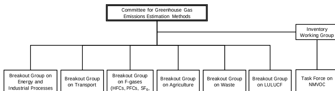
Figure 1-23 Structure of the Committee for the Greenhouse Gas Emissions Estimation Methods
