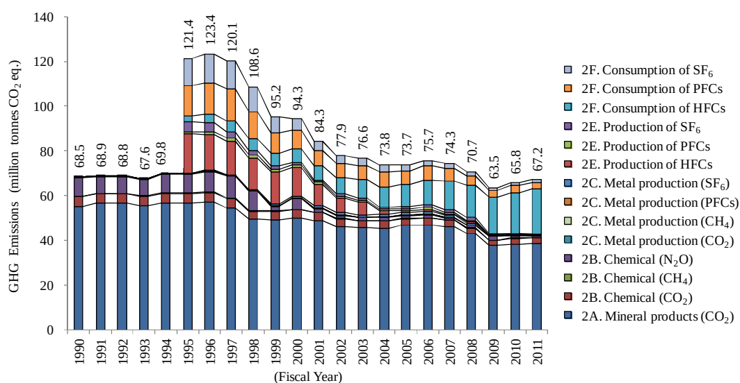
Figure 1-16 Trends in GHG Emissions from the Industrial Processes Sector
