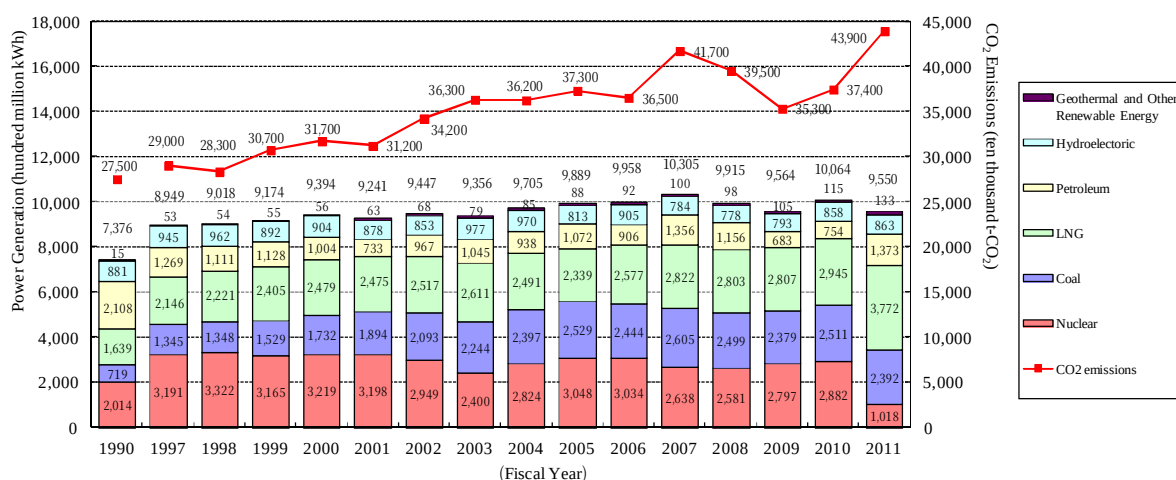
Figure 1-4 The Power Generation by Type and CO 2 Emissions(10 General Electricity Utilities, Including Receiving Power from Other Companies)
