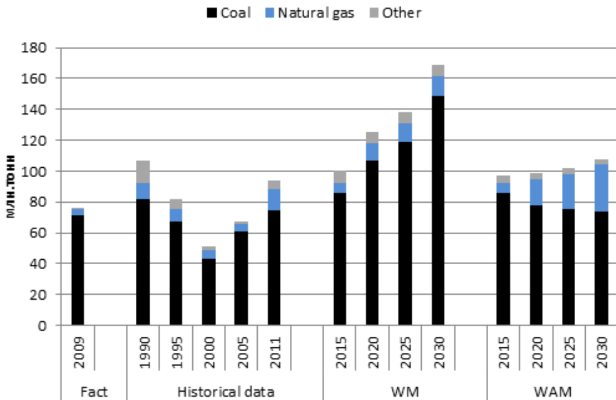
CO 2 emissions related to fuel combustion, at the electric and thermal power plants by fuel types
