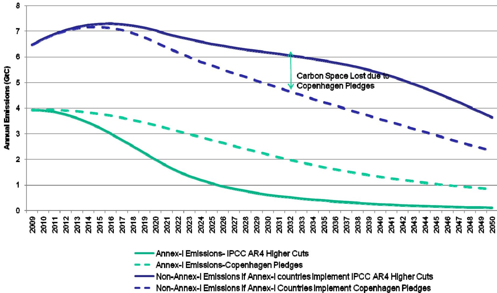
Emission Trajectories for Annex-I and Non-Annex-I Countries - Comparison between Copenhagen Pledges and IPCC AR4 Higher Cuts
