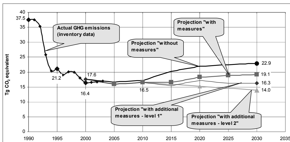
Figure 1. CO 2 emissions projections for the energy sector in Estonia
