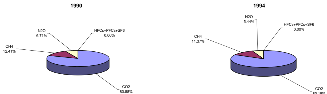
GHG emissions by gas (without LUCF)
