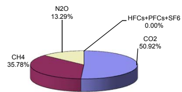
2010 (with LUCF)
