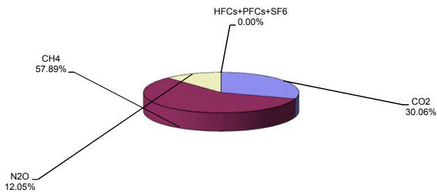
1994 (with LUCF)
