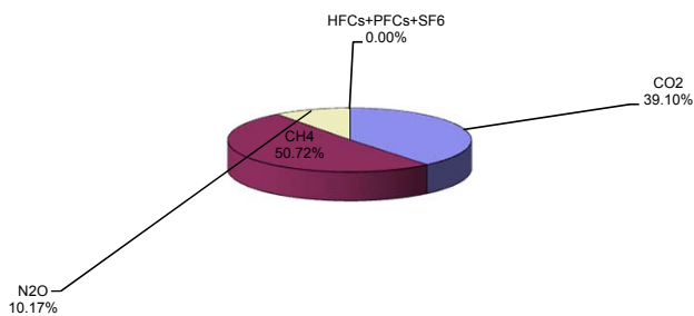
1994 (with LUCF)
