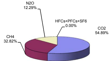
2010 (without LUCF)
