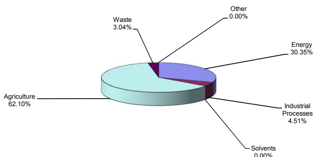
1994
