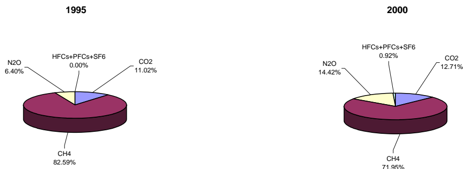
GHG emissions by gas (without LUCF)
