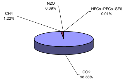
2000 (with LULUCF)
