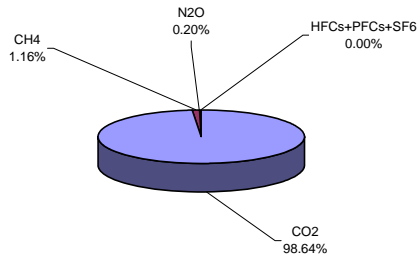
1994 (with LULUCF)
