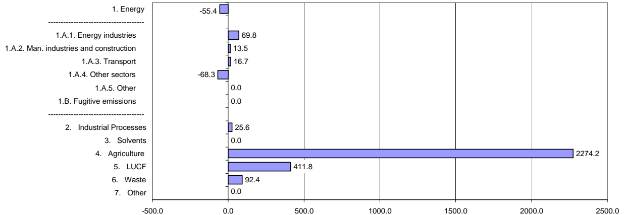
Change in GHG emissions/removals from 1998 to 2005, %
