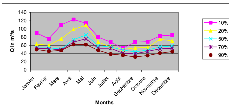
Diag 5: Frequency curves of monthly minima flows at Nyabarongo–Kigali (1974-1990)
