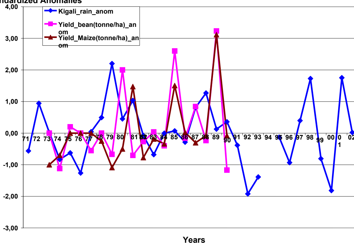
Standardized Anomalies
