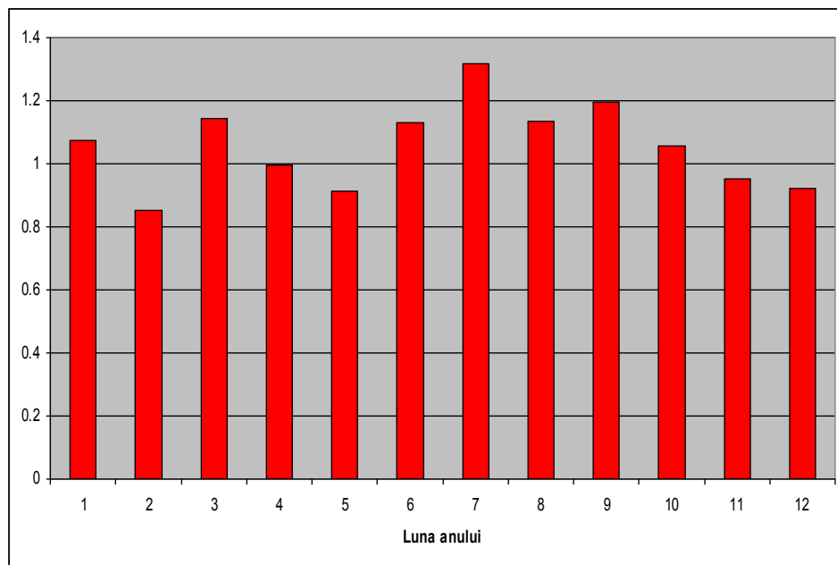
Figure VI_7 Changes of the monthly average temperature ( ^{\circ}\text{C} , left) and the daily ration of precipitations (% , right) for the period 2001-2030 (Scenario A1B) against 1961-1990, as average on Romania. (Values obtained as multimodel average)
