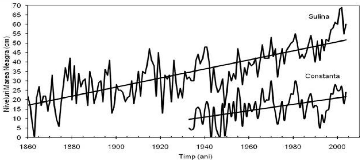
Figure VI_14. Trend of Black Sea level (1860 - 2005)
