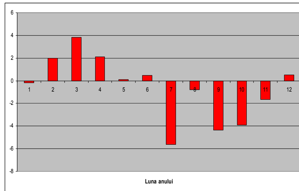
Figure VI_7 Changes of the monthly average temperature ( ^{\circ}\text{C} , left) and the daily ration of precipitations (% , right) for the period 2001-2030 (Scenario A1B) against 1961-1990, as average on Romania. (Values obtained as multimodel average)
