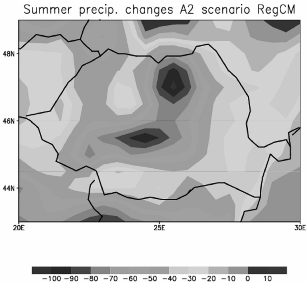
Figure VI_4 Forecasted changes in the precipitation amounts during the summer in Romania For the period 2070-2099 compared to the period 1961-199) achieved with the RegCM model, A2 scenario
