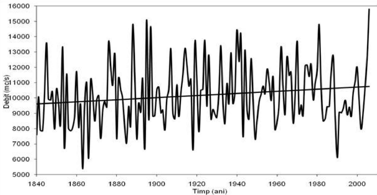
Figure VI_13. Trend of Danube water flow (1840 - 2005)
