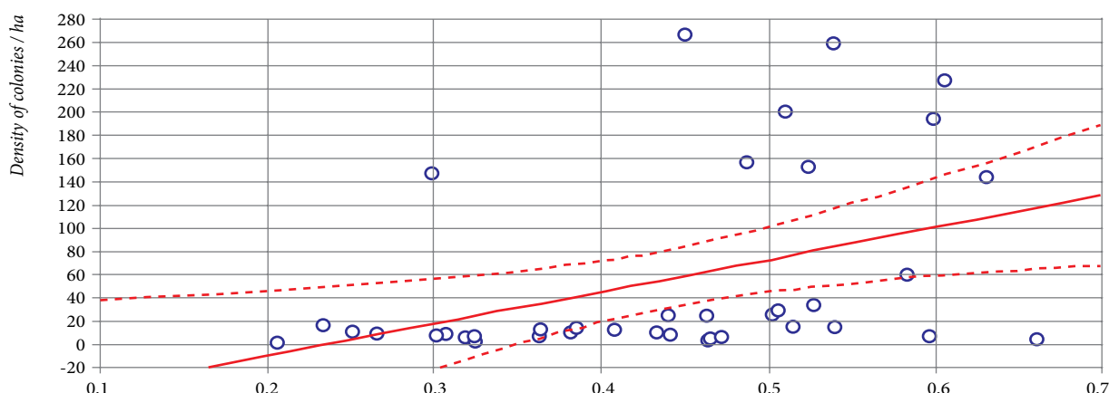
Figure 5-42: Dependence between the density of Microtus arvalis colonies and the Selseaninov's Hydrothermal Coefficient.
