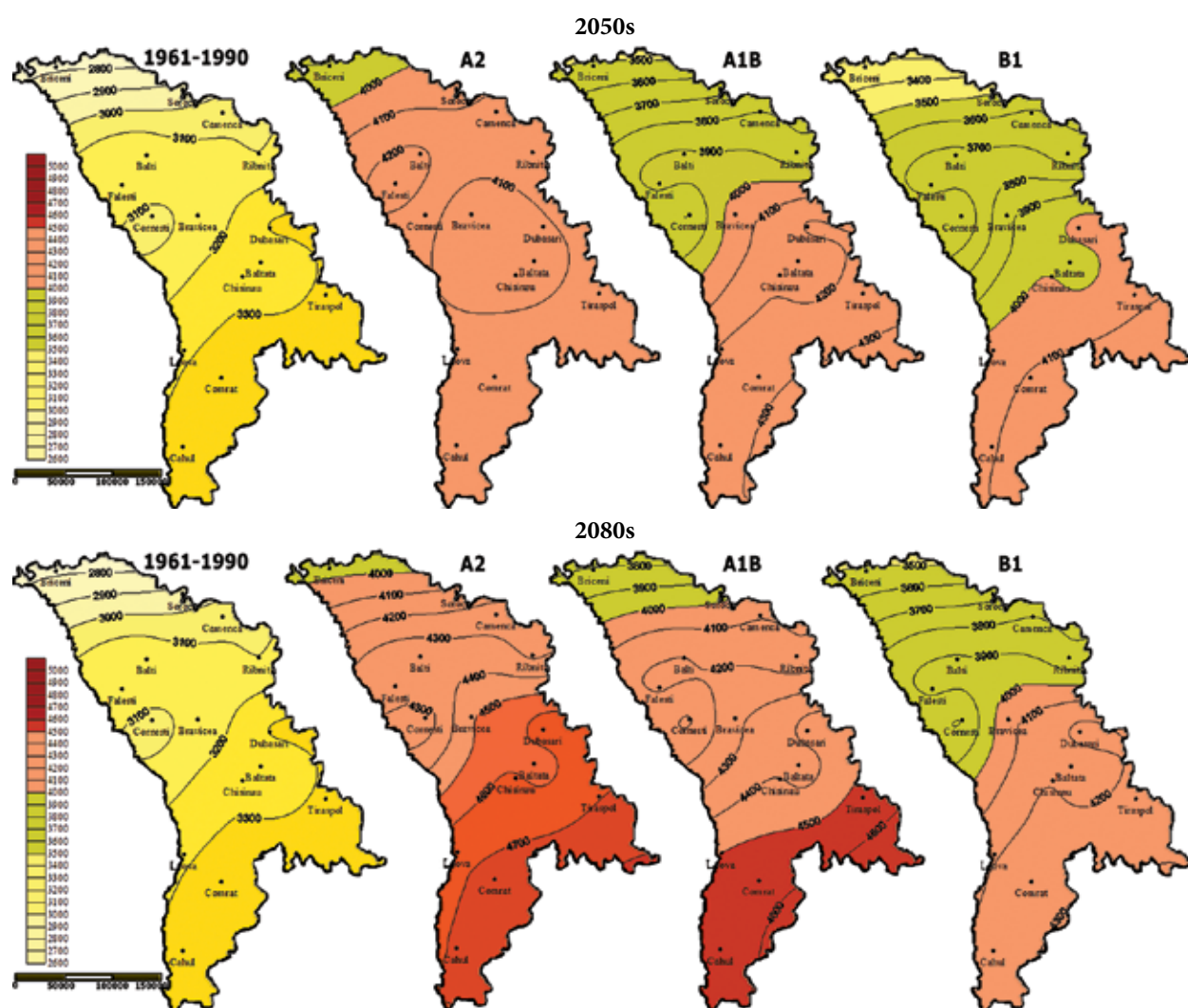
Figure 5-22: Projected Multi - Model Ensemble Sum of Active \Sigma T_{ac>10^{\circ}\text{C}} Temperature, ^{\circ}\text{C} Development throughout the Republic of Moldova 1
