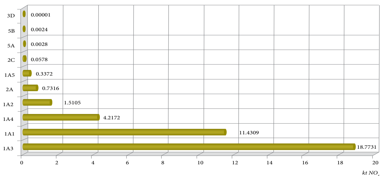
Figure 2-23: 2010 Source Categories of NO x in the Republic of Moldova
