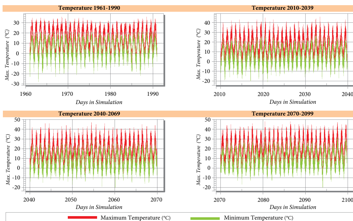
Figure 5-48: The trends of maximum and minimum daily temperatures in RM for the reference period (1961-1990), respectively for the 21 st century: three time periods of 30 years each, focused on the years 2020s, 2050s and 2080s, generated by the PRECIS/ECHAM5 model, imposed by the emissions scenario SRES A1B.
