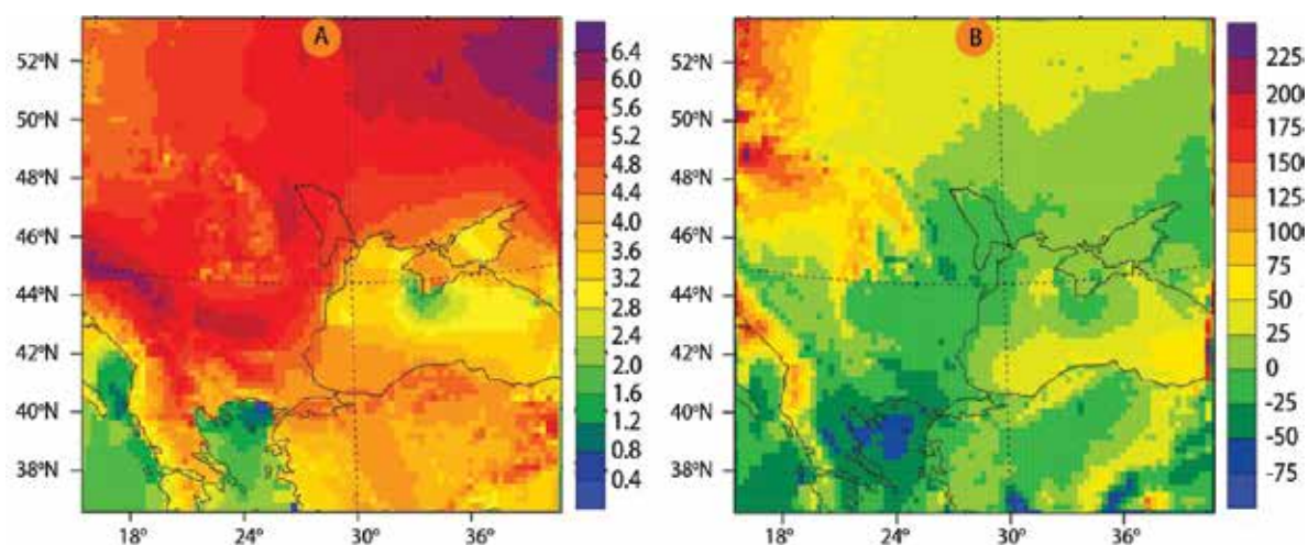
Figure 5-30: Projected PRECIS/ECHAM5 SRES A1B Future Changes in DJF (A) Mean Air Temperature (°C) and (B) Precipitation (%) by 2080s relative to 1961-1990 baseline periods
