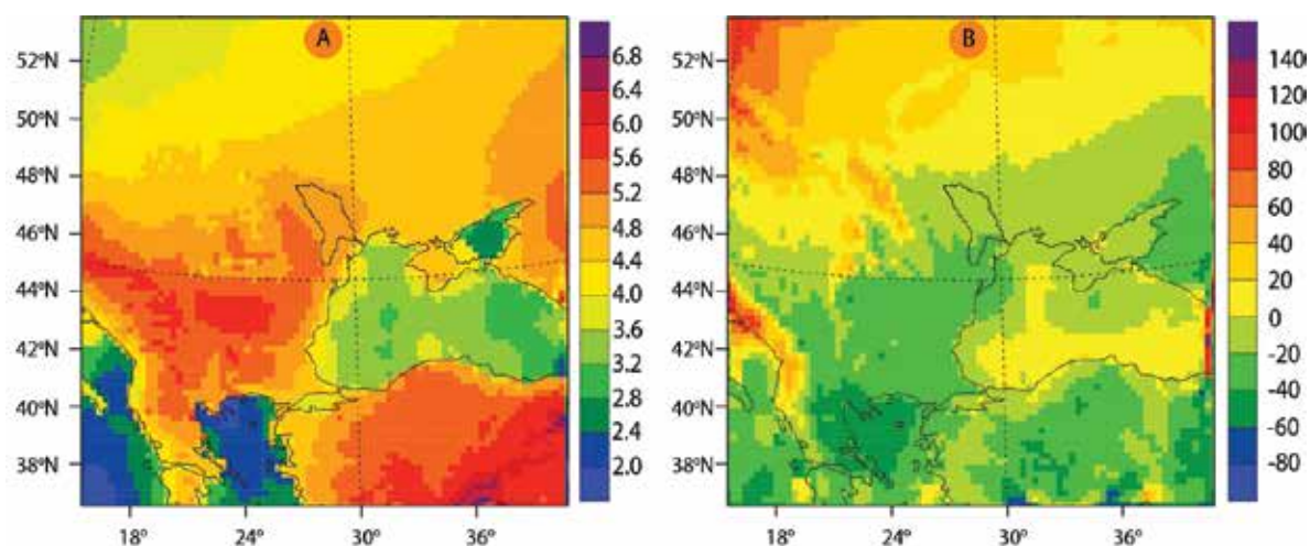
Figure 5-28: Projected PRECIS/ECHAM5 SRES A1B Future Changes in Annual (A) Mean Air Temperature (°C) and (B) Precipitation (%) by 2080s relative to 1961-1990 baseline periods
