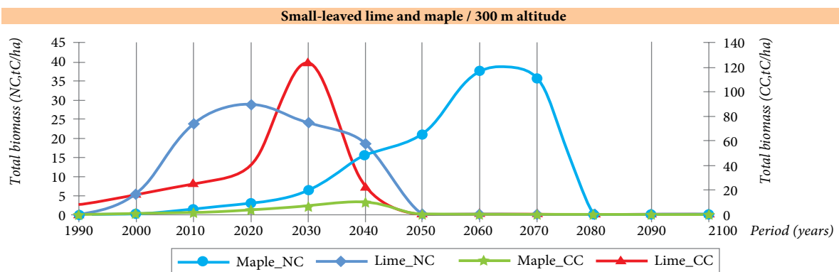
Figure 5-40: Prospects of relative biomass accumulations for the small-leaved lime (tC/ha) in RM in the 21 st century (the Climate Change Scenario) as compared to the climate conditions typical for the 1961-1990 period (the Normal Climate Scenario), according to an ensemble of 10 global climate models imposed by the emission scenario SRES A1B.
