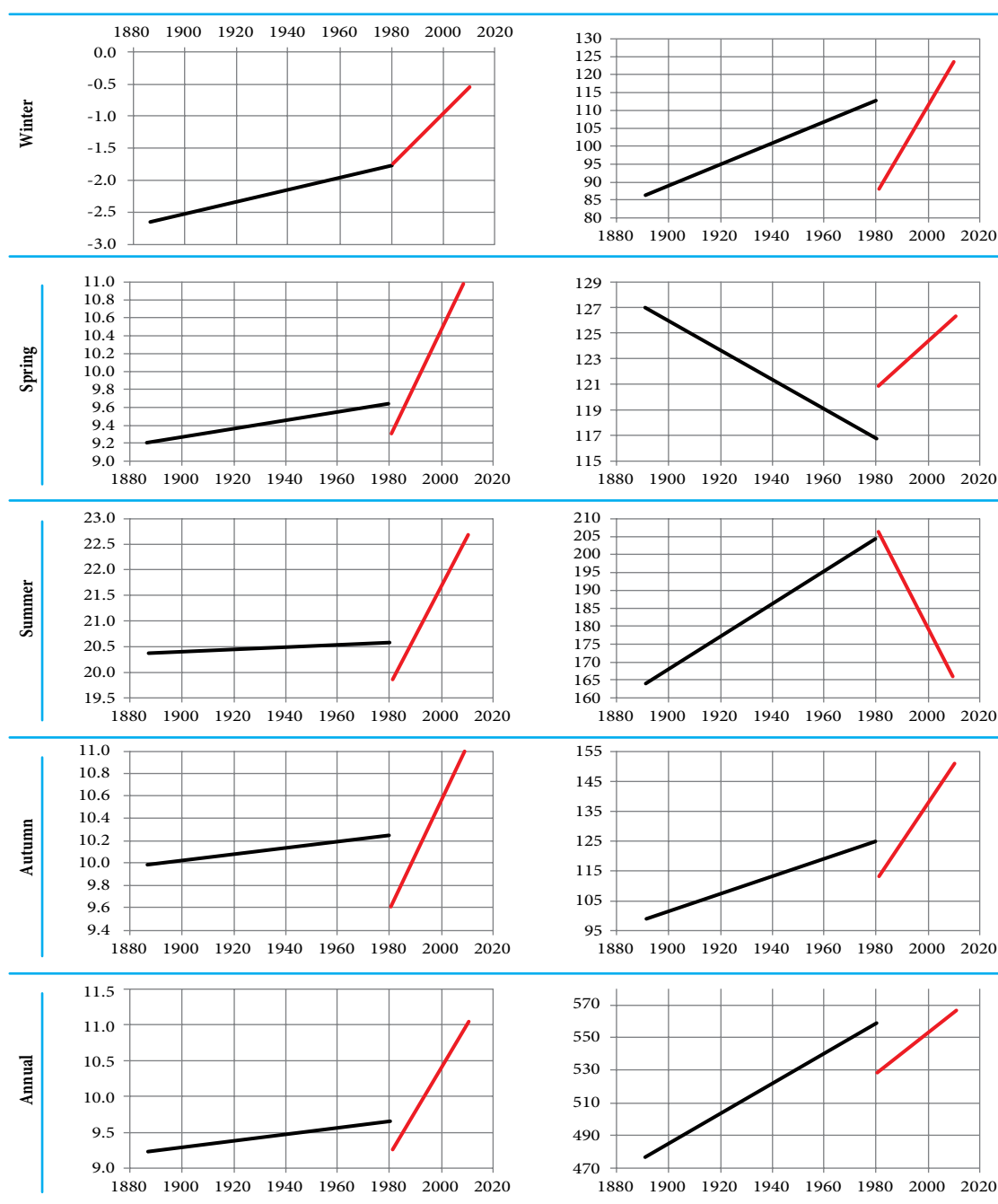
Figure 5-11: Trends in average air temperature ( ^{\circ}\text{C}/\text{year} ) – left side, and precipitation ( \text{mm}/\text{year} ) – right side, for the period before 1981 year and beyond, at the Chisinau Meteorological Station
