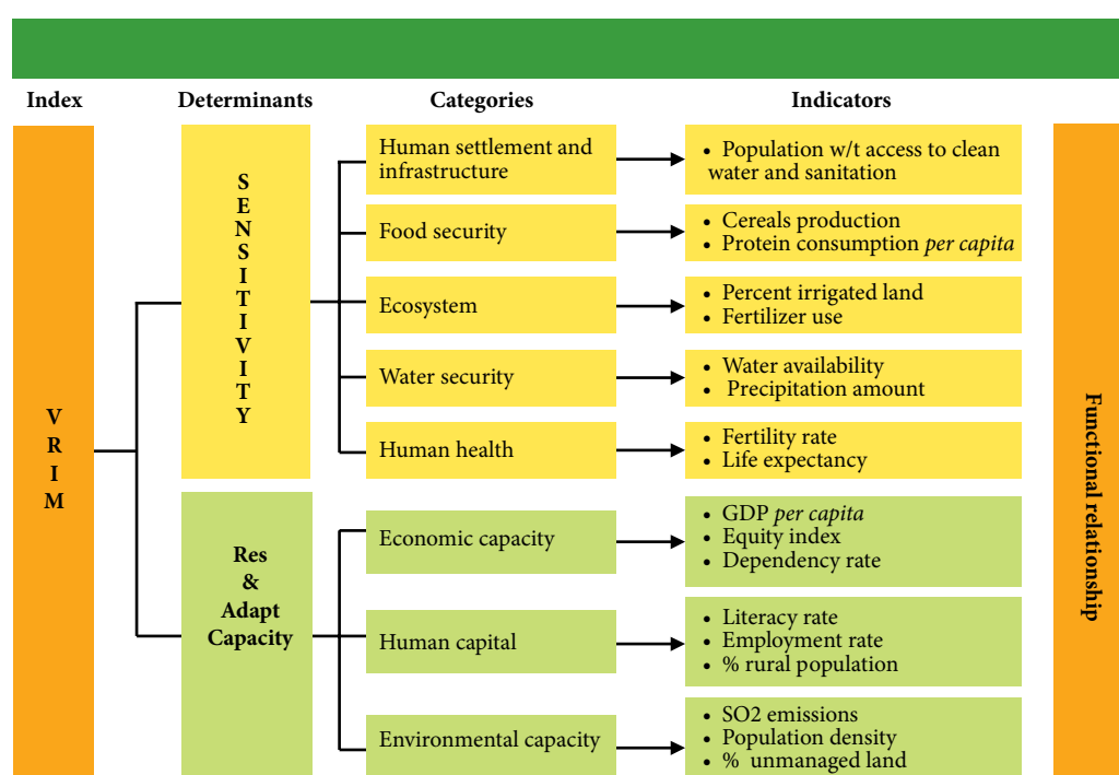
Figure 5-1: Vulnerability and Resilience Indicators Model (VRIM) used as prototype in developing the CVI for the Republic of Moldova.
