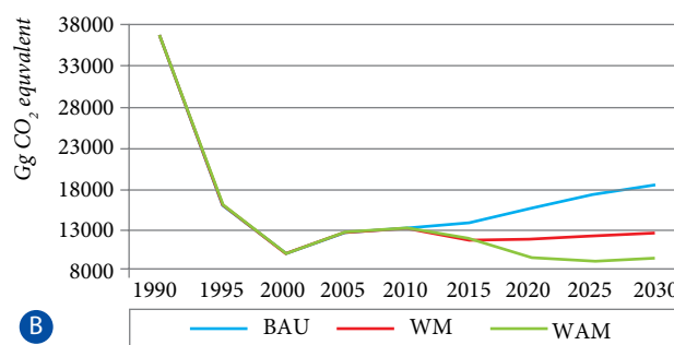
Figure S-5: Projections of total GHG emissions under the considered scenarios in the RM, for the period up to 2030: (a) without LULUCF; (b) with LULUCF
