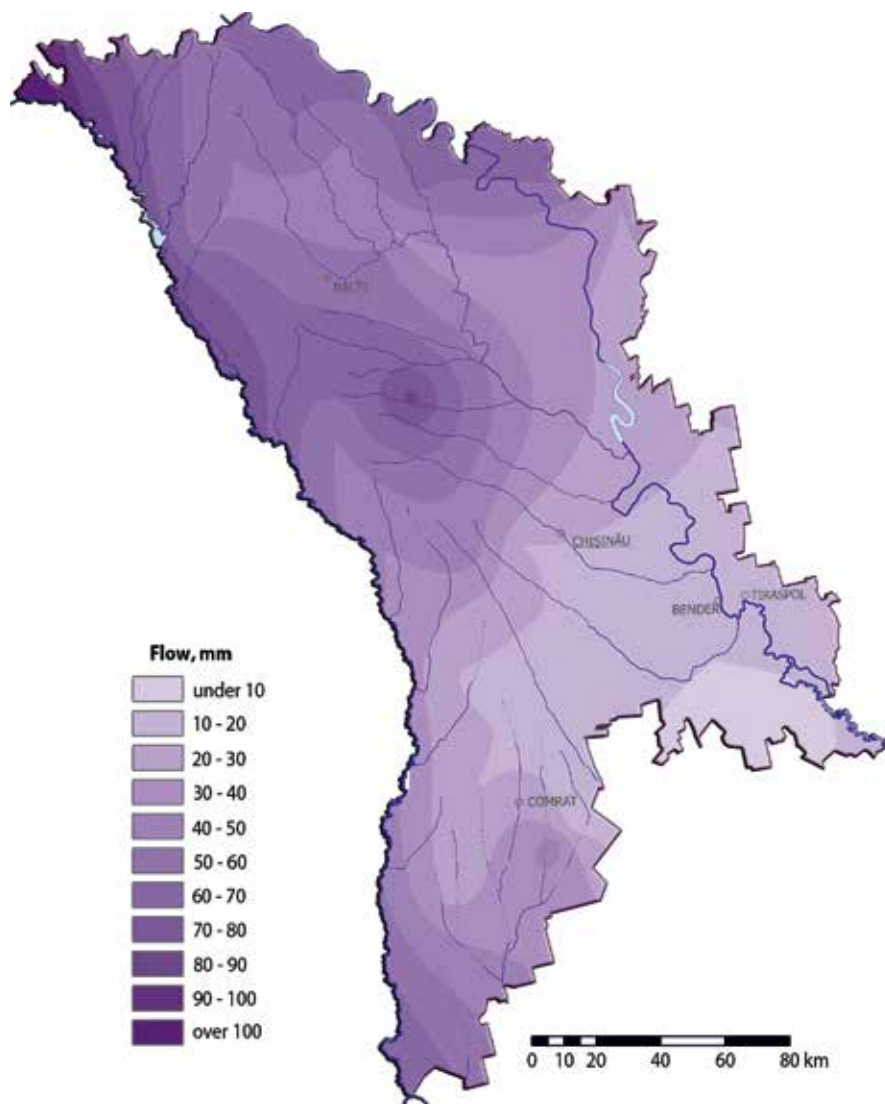
Figure 5-53: Layer of multiannual average flow, mm
