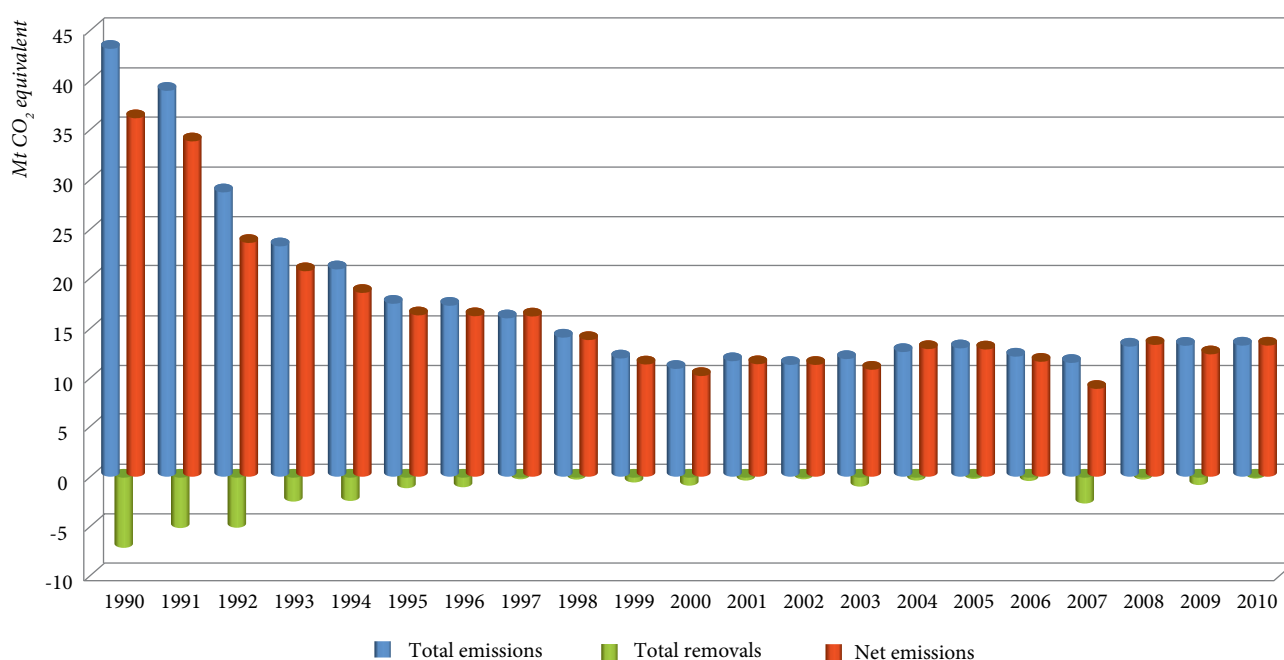
Figure 2-6: Greenhouse Gas Emission and Sink Trends in the Republic of Moldova, 1990-2010
