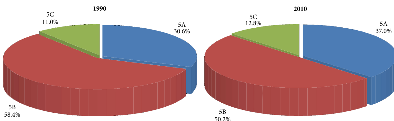
Figure 2-20: Breakdown of GHG Emissions and Removals by source and sink categories in LULUCF Sector, in 1990 and 2010
