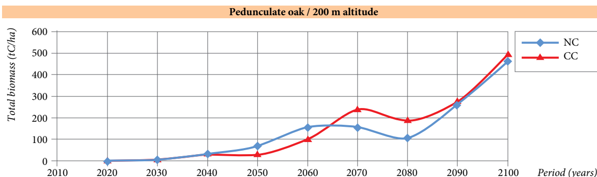
Figure 5-41: Prospects of relative biomass accumulations for pedunculate oak (tC/ha) in RM in the 21 st century (the Climate Change Scenario) as compared to the climate conditions typical for the 1961-1990 period (the Normal Climate Scenario), according to an ensemble of 10 global climate models imposed by the emission scenario SRES A1B.
