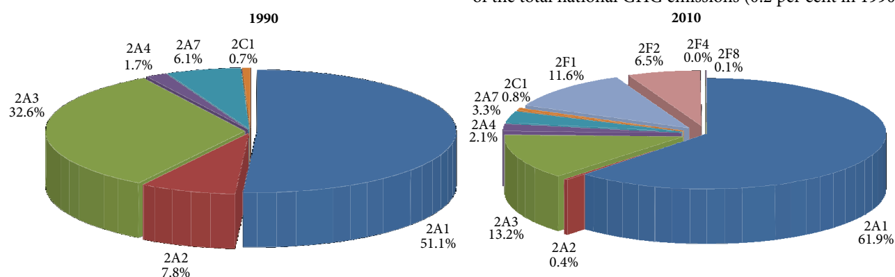
Figure 2-15: Breakdown of Industrial Processes' GHG Emissions by Category in 1990 and 2010
