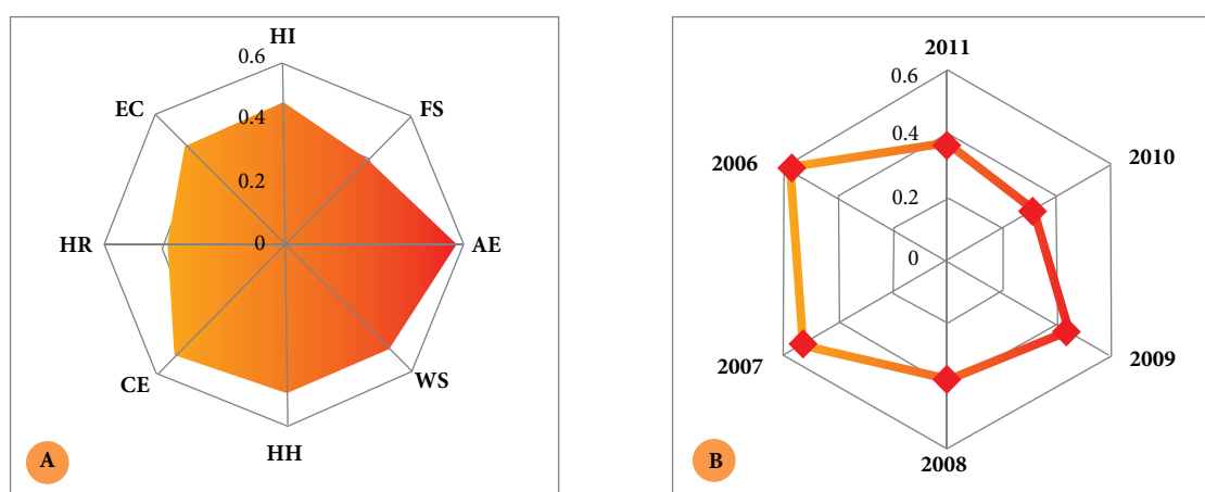
Figure 5-4: Climate Vulnerability Index of the RM (CVIM) for 2006-2011 at national level on the basis of categories (A) and values for each year (B), where: HI – housing infrastructure, HH – human health, FS – food safety, WS – water supply, AE – agricultural ecosystems, EC – economic capacity, EC – environmental capacity, HR – human resources.
