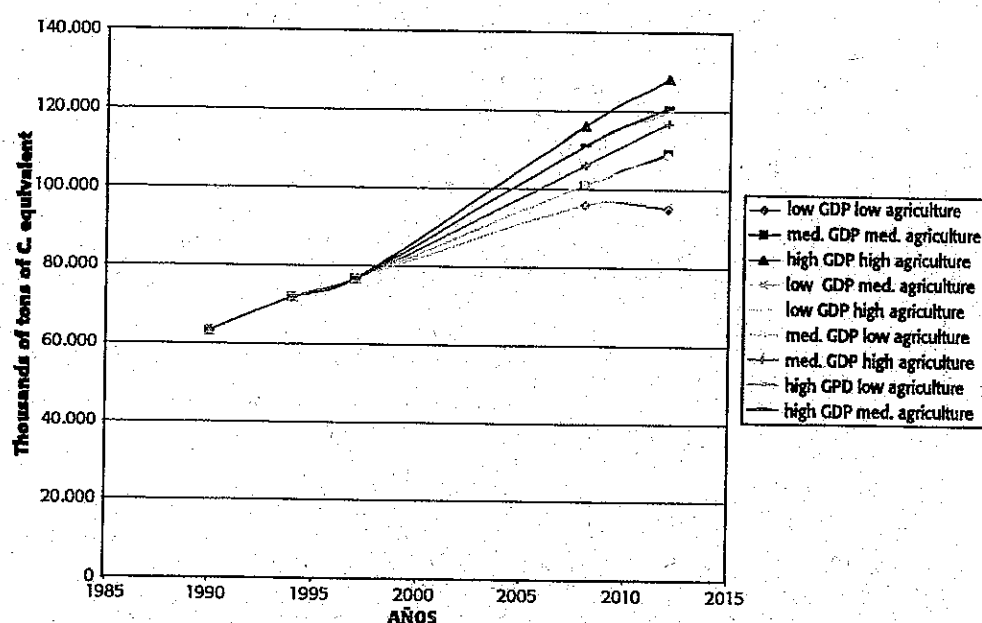
Figure 4.2. GHG Emissions.
