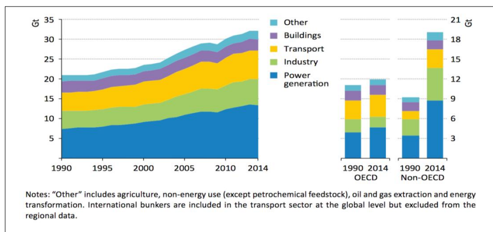
Figure 1 Global energy-related carbon dioxide emissions by sector and region
