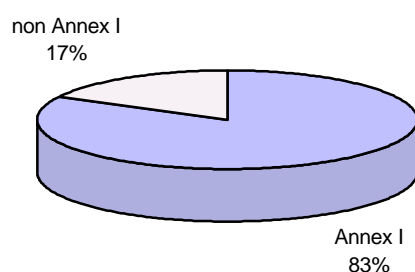
Figure 7 - Relative responsibility attributable to each group of Parties, according to induced temperature increase in 2010 due to CO2 emissions.
