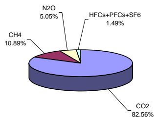
1990 (with LULUCF)
