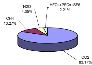
2009 (with LULUCF)
