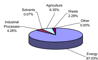
2009
