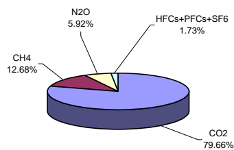
1990 (with LULUCF)
