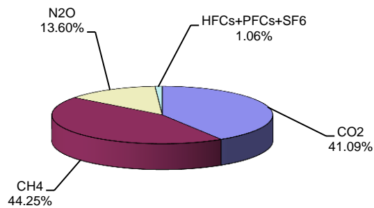
1990 (with LULUCF)
