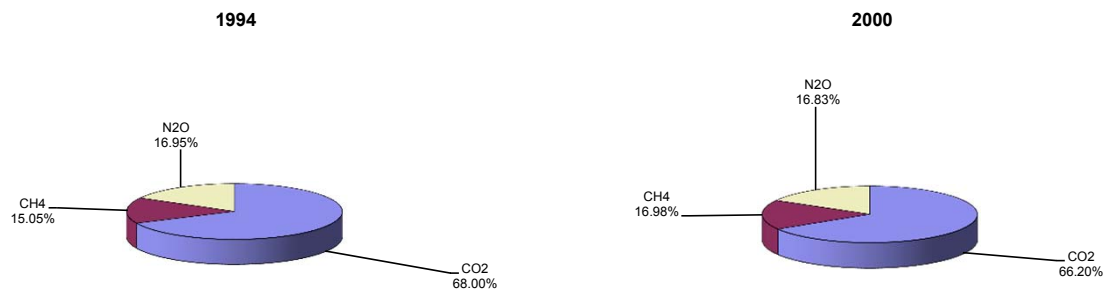
GHG emissions by gas (without LUCF)
